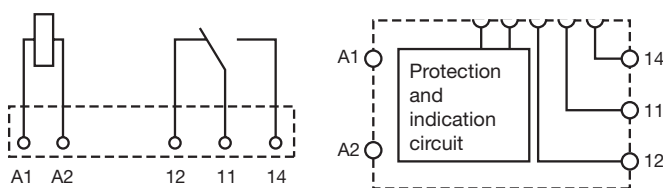
Circuit / Terminal Layout:
